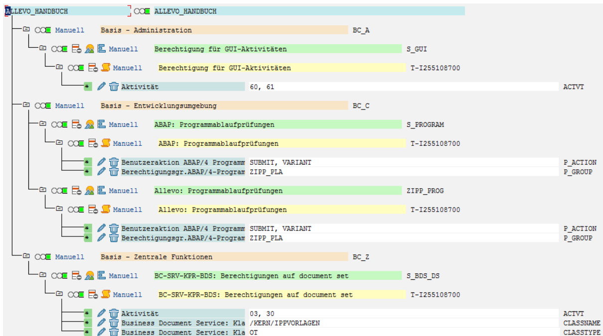
Figure 26-1: Role with authorization objects for planners
