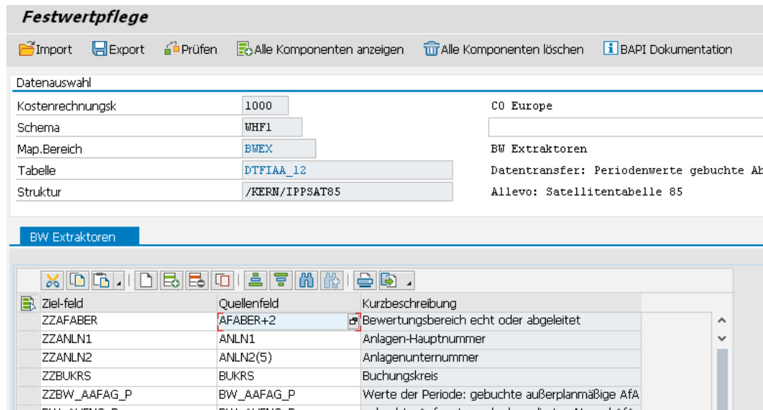
Figure 17-23: DataSource field mapping
