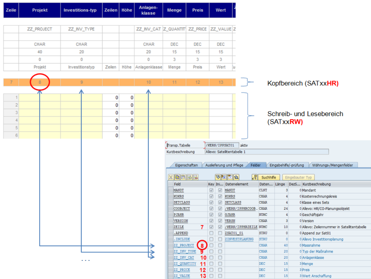
Figure 16-2: Append structure of the SAP table and Excel names of the satellite tables
