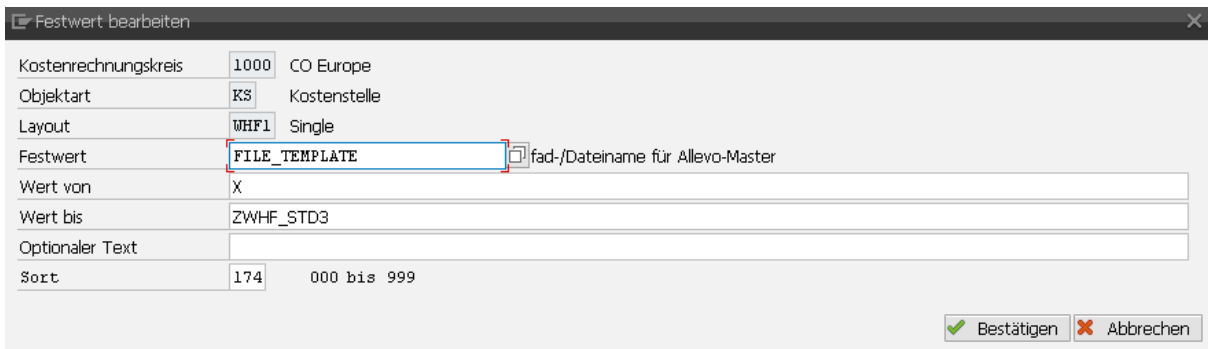
Figure 7-4: Edit Allevo constant
