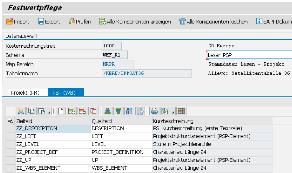
Figure 17-32: Field assignment for reading data to the project
