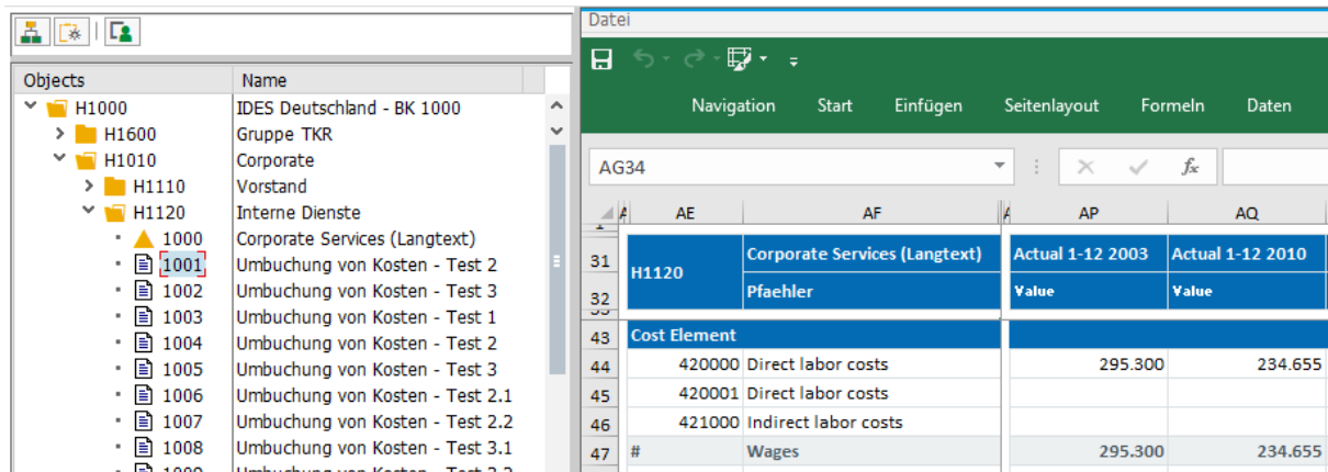
Figure 3-14: Reading to the cost center group in the Inplace tree
