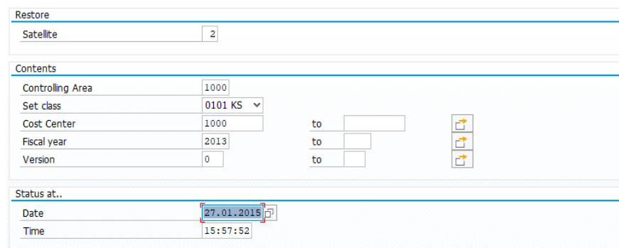
Figure 16-8: Restore data to the satellite
