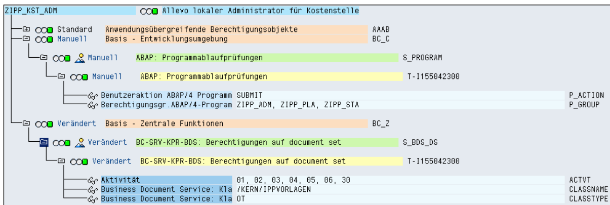
Figure 26-3: Example for the permissions of a local administrator
