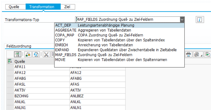
Figure 19-2 Allevo Orbit Transformation with field mapping
