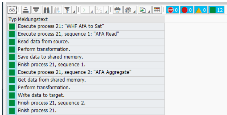
Figure 19-6 Allevo Orbit execution protocol with two steps
