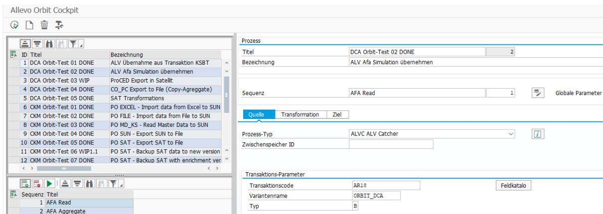
Figure 19-1: Allevo Orbit initial screen
