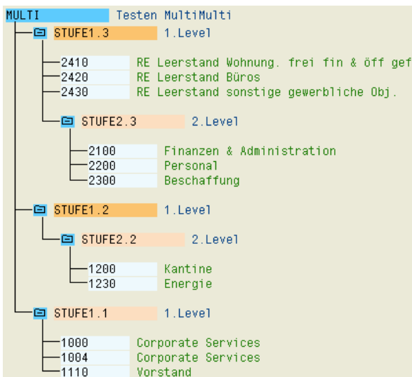
Figure 21-3: Group with more than 2 levels
