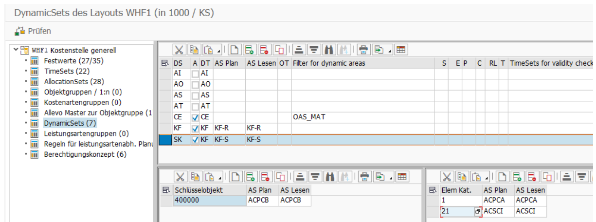
Figure 7-19: Settings for DynamicSets
