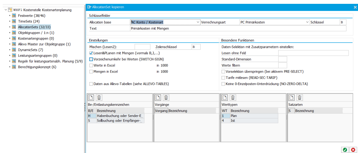
Figure 7-16: Properties of the AllocationSet
