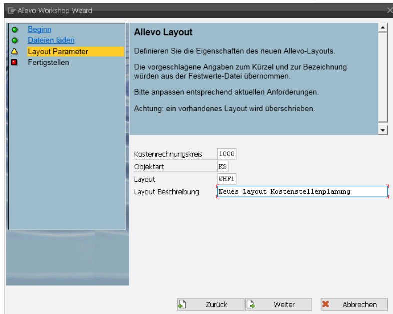
Figure 9-3: Allevo Assistant for creating Allevo layouts
