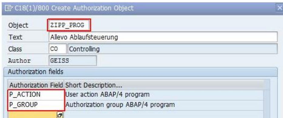
Figure 26-2: Create authorization object ZIPP_PROG in SU21
