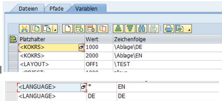
Figure 30-1: Placeholder and assigned strings
