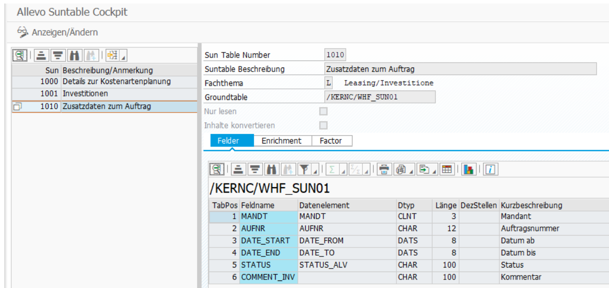
Figure 18-1: Cockpit for SunTables
