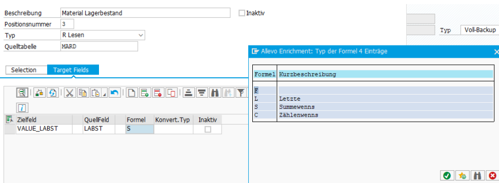
Figure 17-42: Data enrichment with "Sum" function
